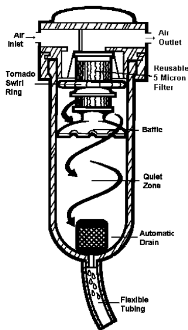
Figure 1 - Air Filter
